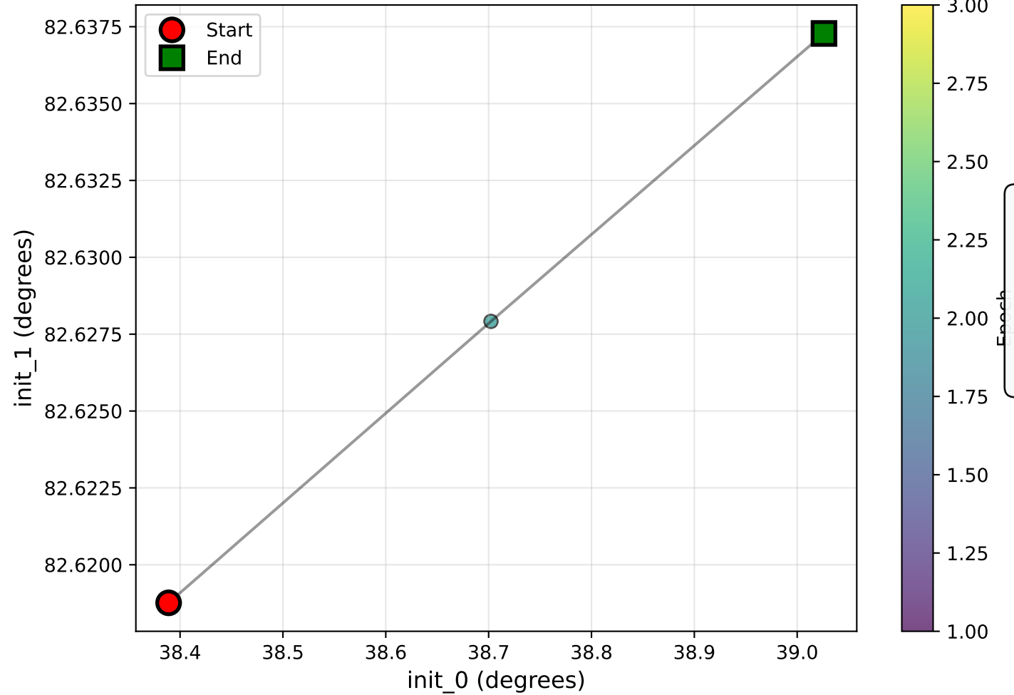
Optimization Trajectory
