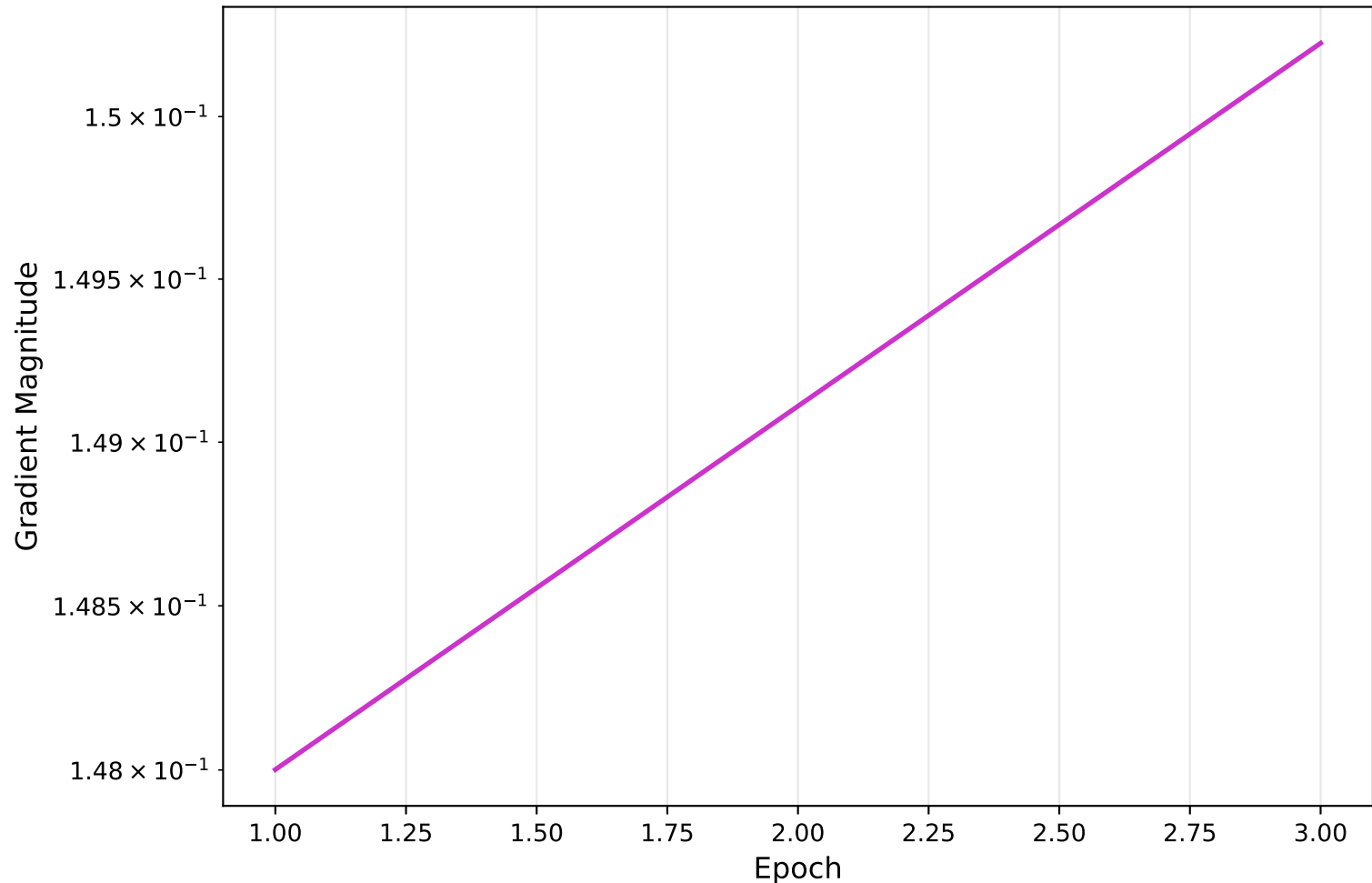
Optimization Dashboard
